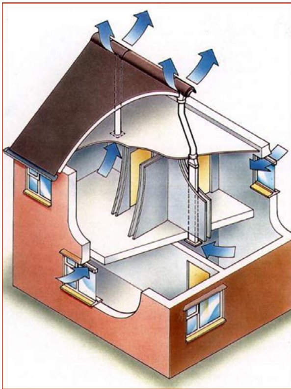
Passive Stack Ventilation Picture Credit: John Willoughby
