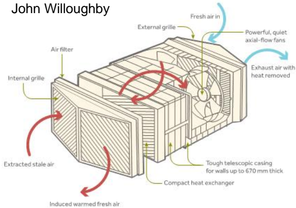
Schematic for Heat Recovery Room ventilator (HRRV) Picture Credit: John Willoughby
