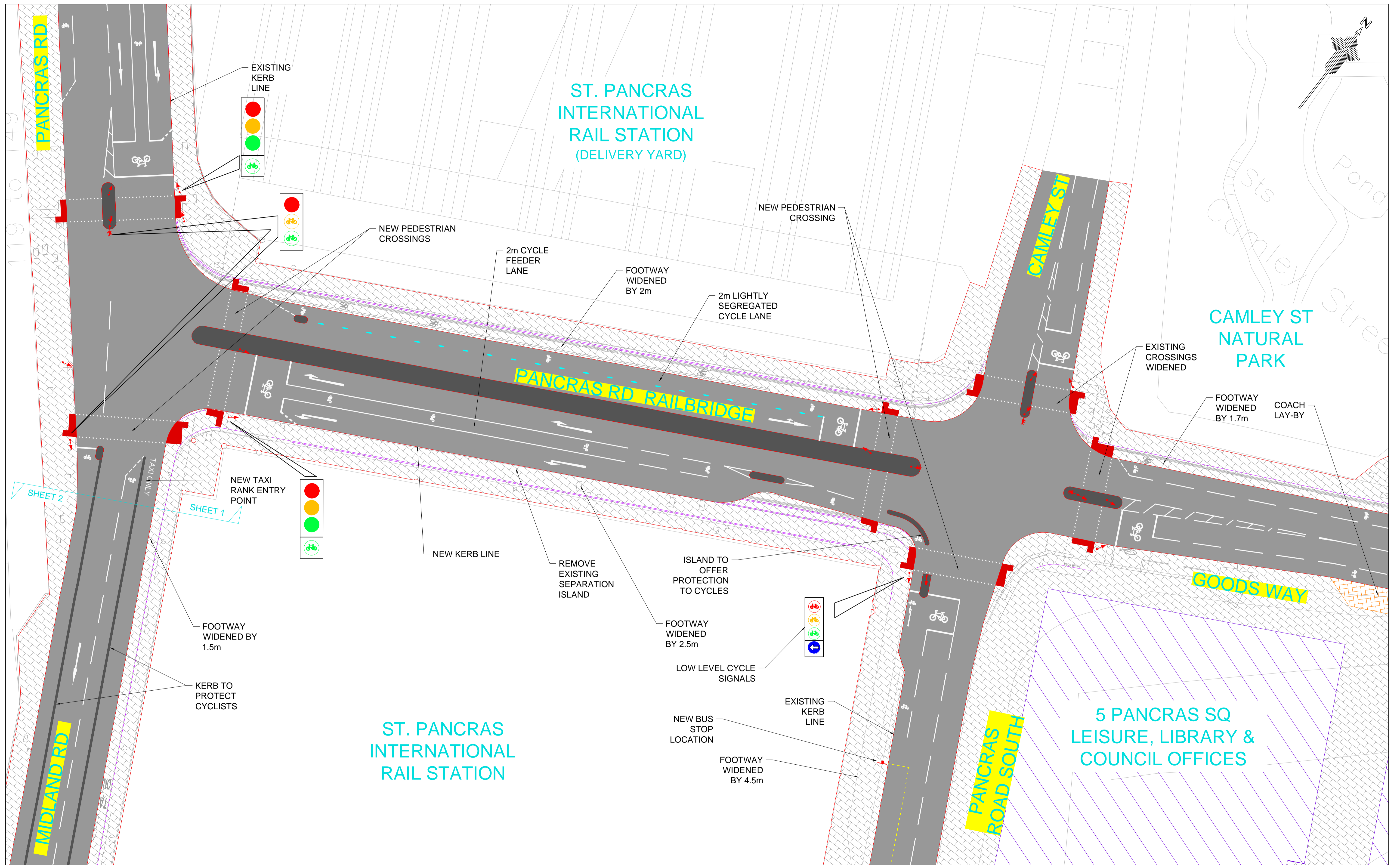
PANCRAS RD RAIL BRIDGE / GOODS WAY / CAMLEY ST. & PANCRAS RD / MIDLAND RD JUNCTIONS PROPOSED WALKING & CYCLING IMPROVEMENTS SHEET 01 OF 02
